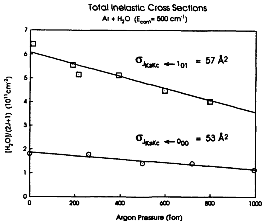
Fig. 4. Ar + H 2 O scattering at E_{\text{com}} = 500 \text{ cm}^{-1} . The \square and \circ represent total loss out of the 1_{01} (ortho) and 0_{00} (para) levels of water, respectively.
